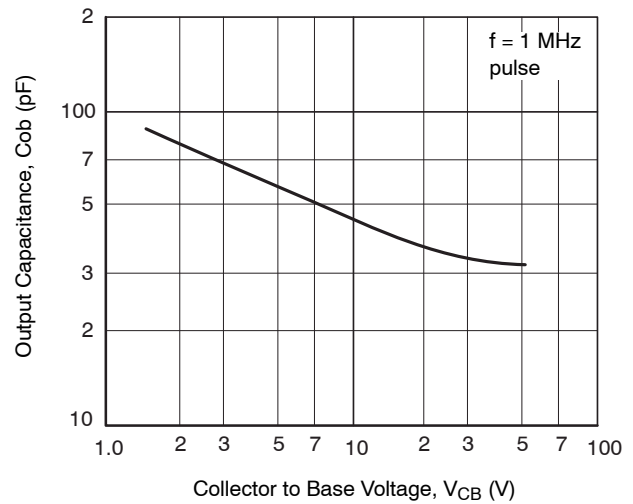
Figure 6. C_{ob} - V_{CB}
